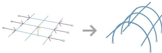
Figure 9 Gridshell schema and the ready model
