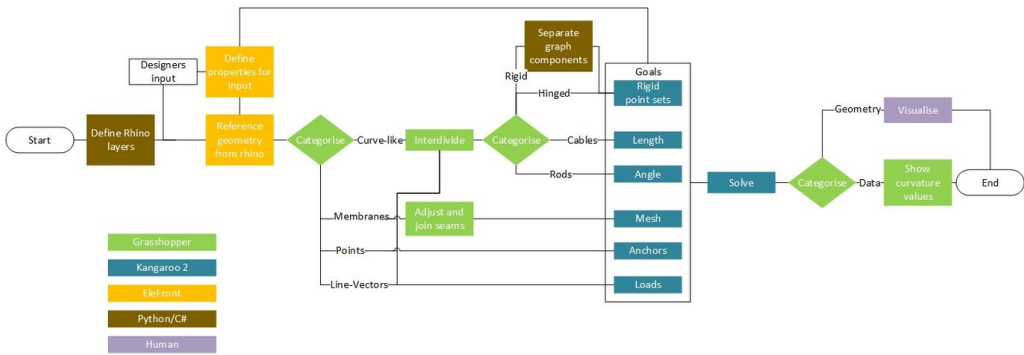
Figure 8 Macro process flow chart of the algorithm
