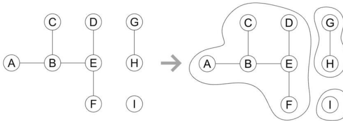
Figure 3 Graph connected components clustering
